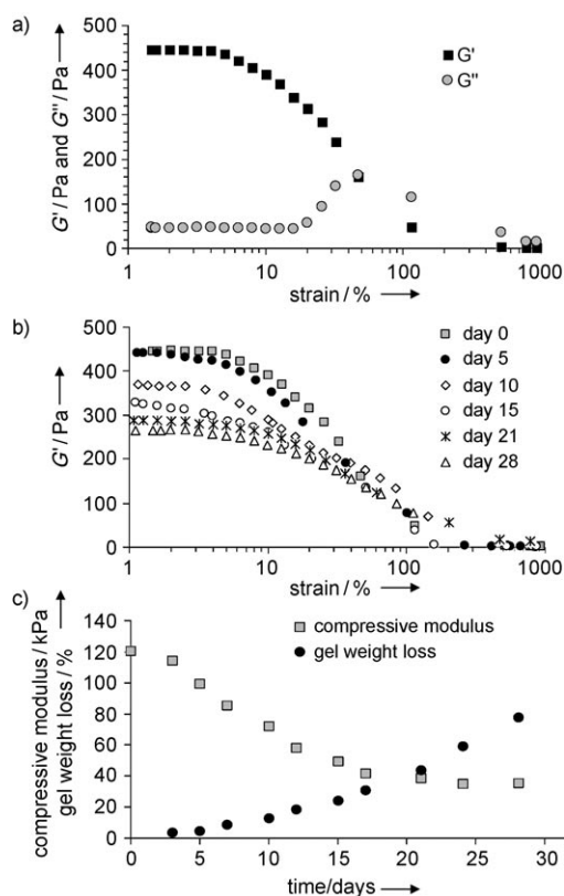
Figure 3. Mechanical and degradation properties of the chitosan/PEI 40:60 hydrogel (all measurements were conducted at 37 °C). a) Storage modulus ( G' ) and loss modulus ( G'' ) plotted as a function of strain. b) Storage modulus versus strain (%) over time and c) compressive modulus and weight loss as a function of time (gel samples for all these studies were 1 cm (height) \times 2 cm (diameter)).
