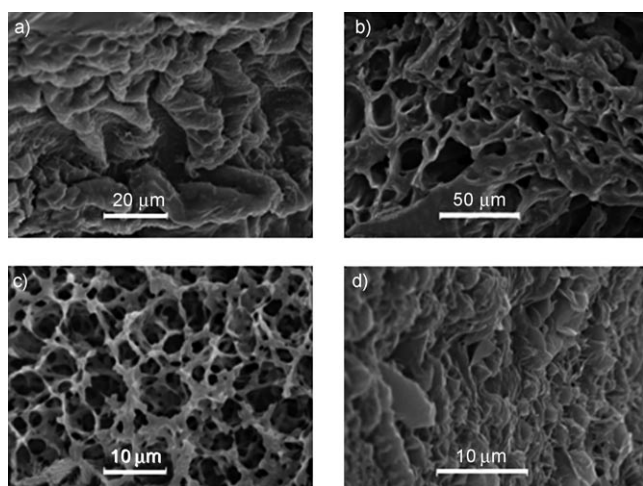
Figure 2. SEM images of hydrogels frozen in liquid nitrogen and freeze-dried: a) chitosan/PEI (10:90), b)–c) chitosan/PEI (40:60) and d) chitosan gel (chitosan solution neutralized with NaOH).
